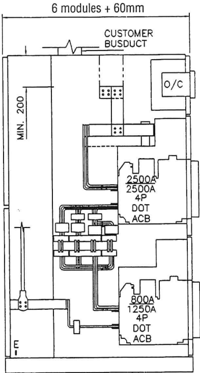
SECTIONAL VIEW FOR CABLE AND BUSBAR ENTRY FROM TOP 剖视图见密封母排及电缆接法
