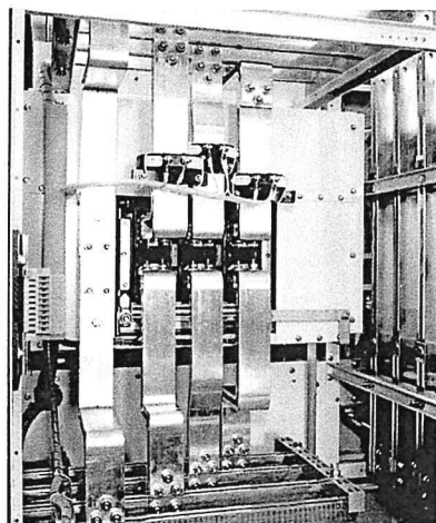
Sectional ACB with upper and lower Busbar connected. 母联 ACB 与上下母线的连接。
