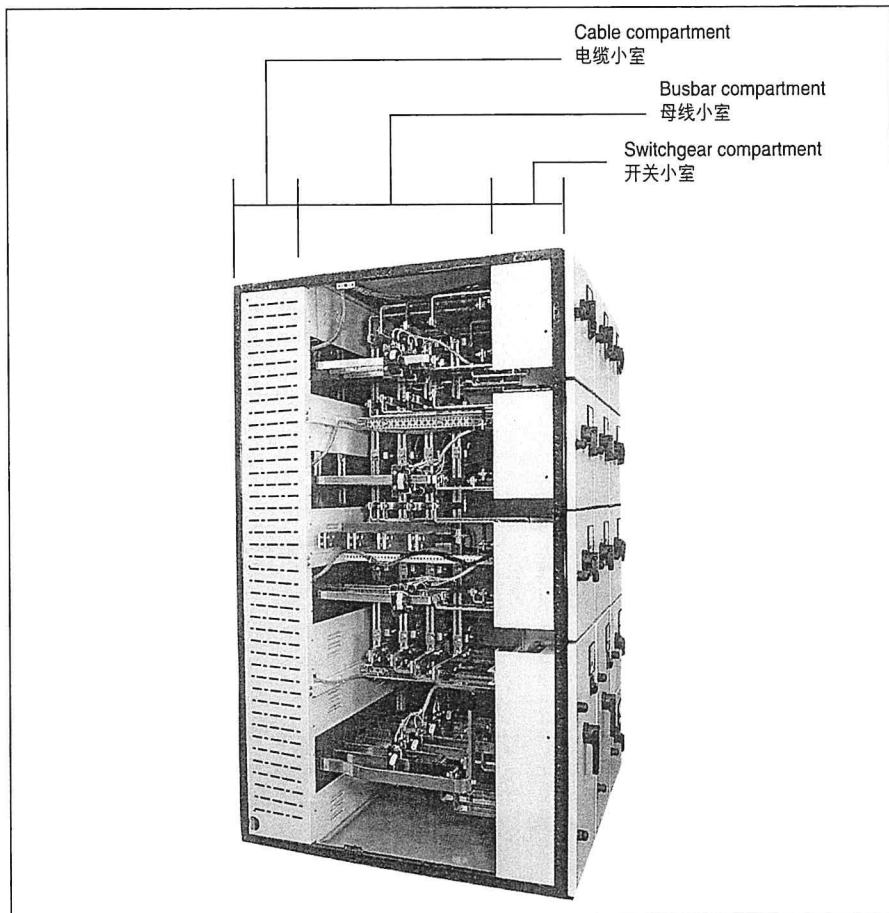
ABB MD190 (HONOR) switchboard side view showing clear the switchgear compartments, busbar compartments and cable compartments. (Standard Form 3b design)
