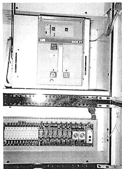
Provide suitable switchgear and control compartment. 2500A ACB 开关小室及控制小室。
