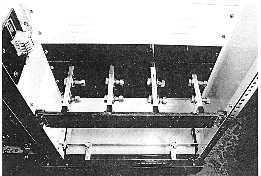
Cabling compartment suitable for cable and busbar coming from top or bottom. 方便底顶出线的母线小室。
