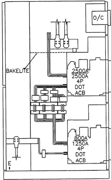
SECTIONAL VIEW FOR CABLE ENTRY FROM TOP AND BOTTOM 剖视图见上位及下位进出电缆接法
